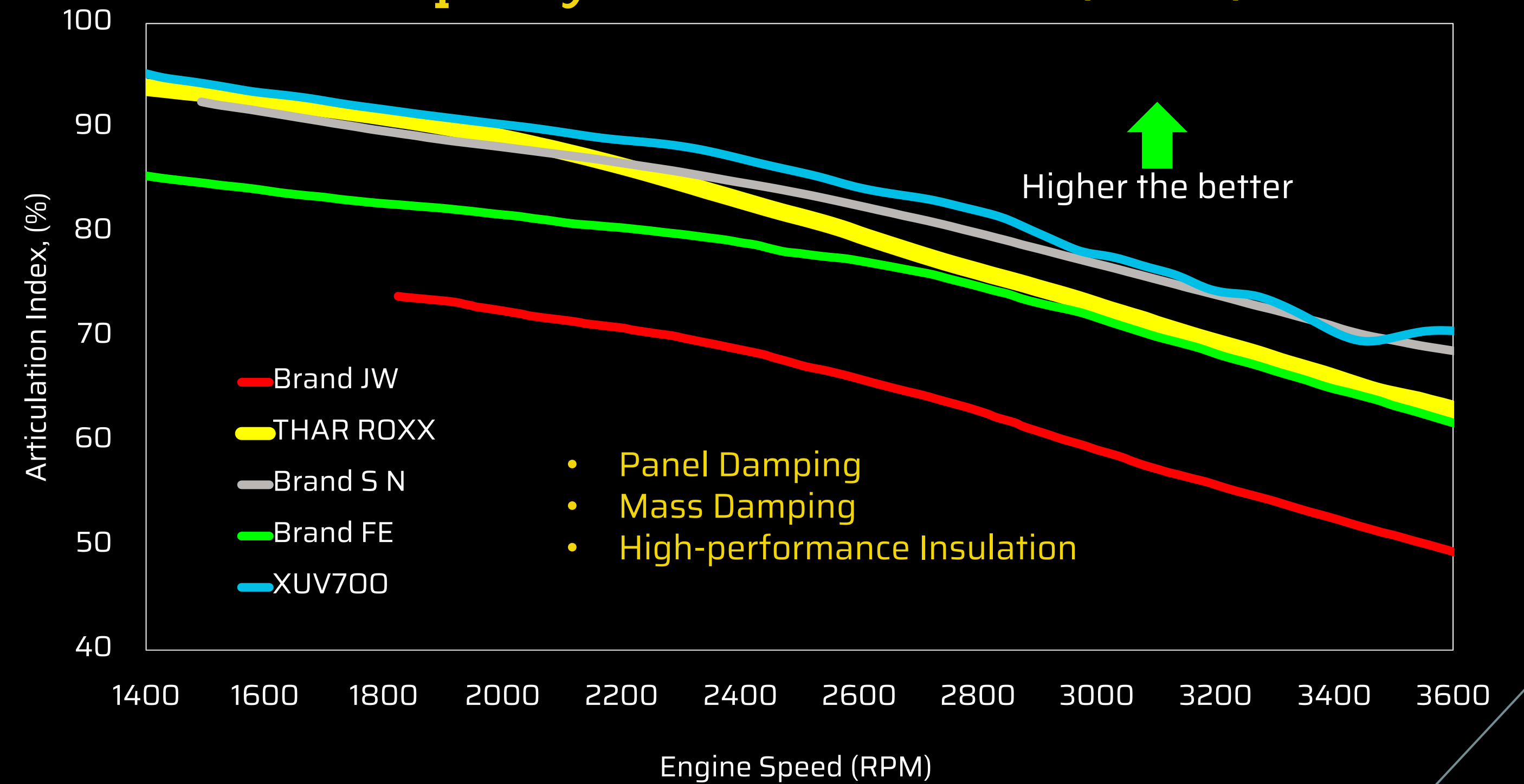
Sound quality : Articulation Index (Diesel)
